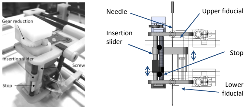
Fig. 2. Stop mechanism for setting the insertion stroke
