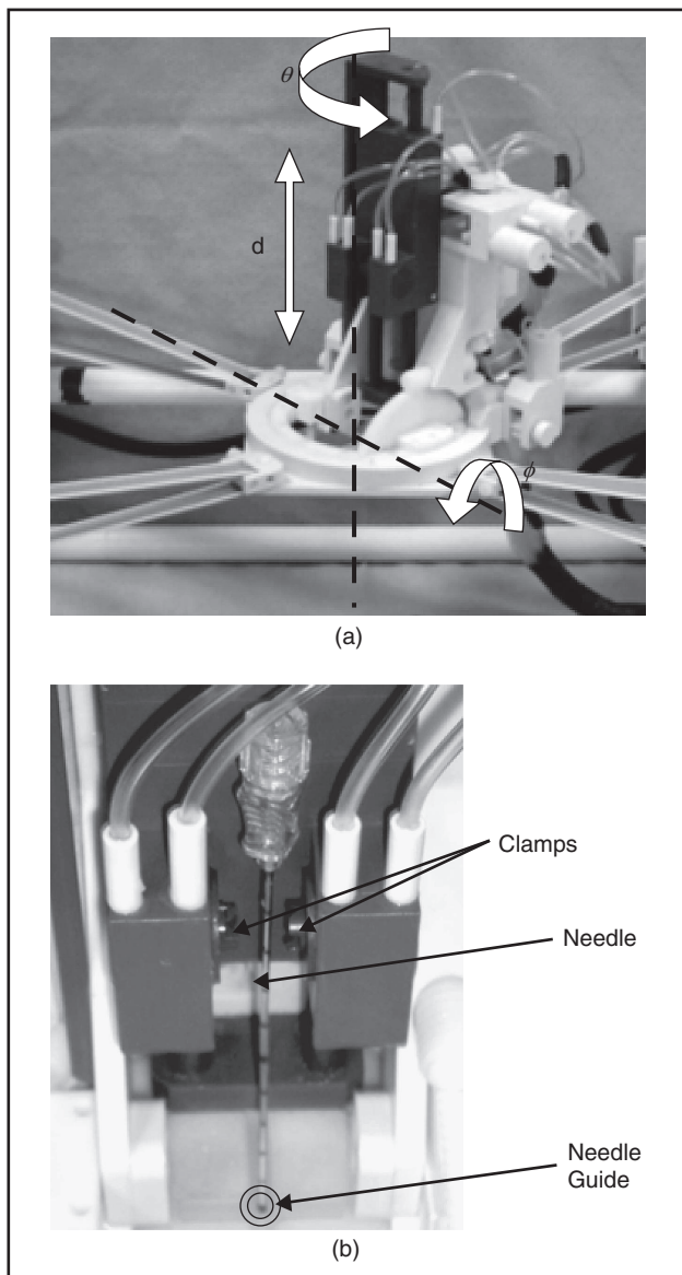
Fig. 2. The LPR needle holder. (a) DoF of the needle holder. (b) The needle-holder puncture part.
