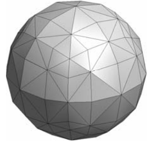
Fig. 1. Equivalent rational ball of a 3D 5 \times 5 \times 5 isotropic chamfer mask.
