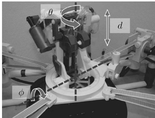
Fig. 3. Needle-holder DoFs.
