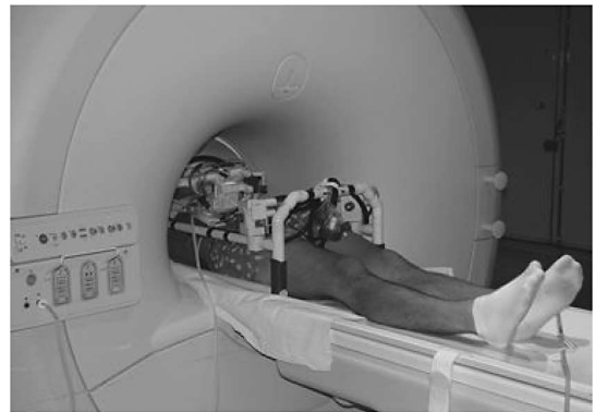
Fig. 1. Photograph of the LPR robot on patient inside MRI device.
